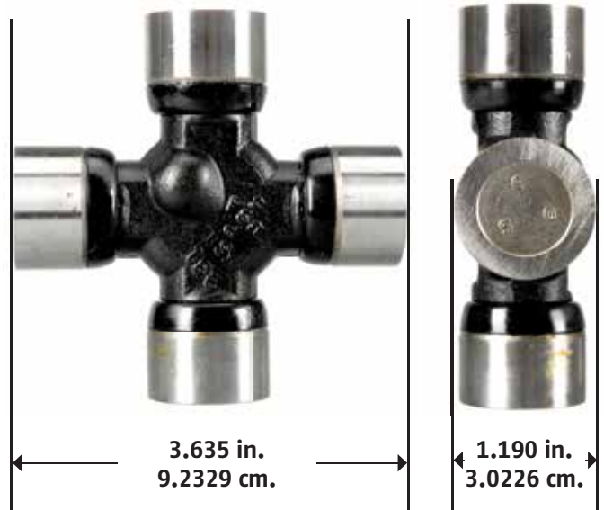
627-185* Half Shaft AC Delco-Non-Greasable
