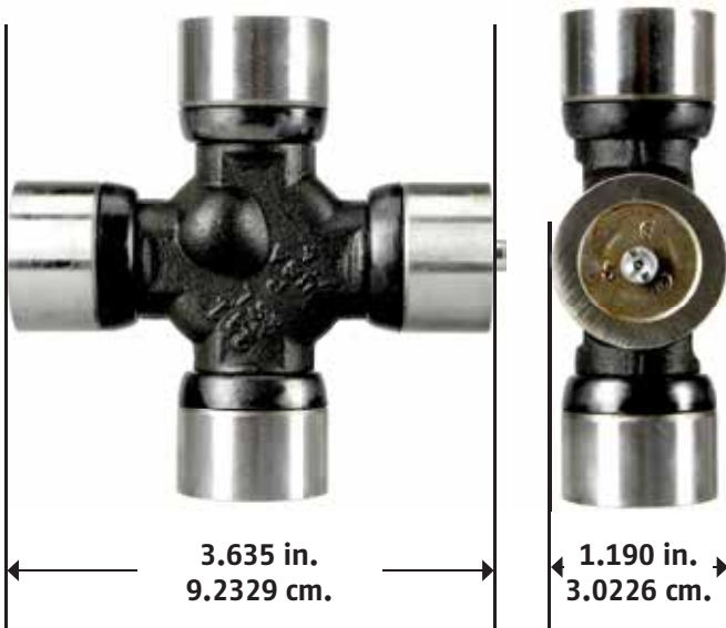
627-184* Half Shaft AC Delco-Greasable End Cap
