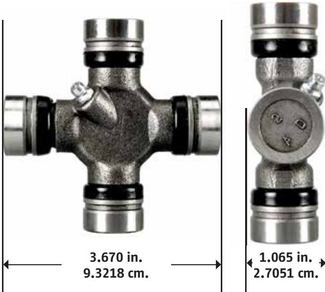
602-916 Drive Shaft Replacement-Greasable
